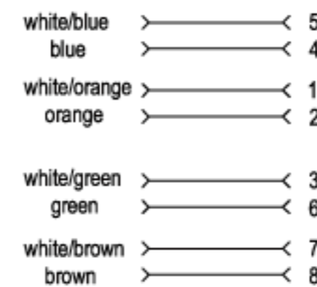
Electrical schematic T568B
