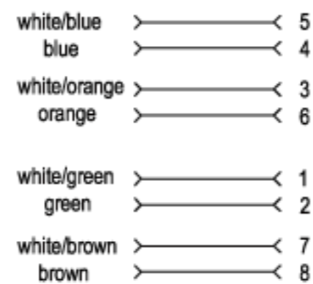
Electrical schematic T568A
